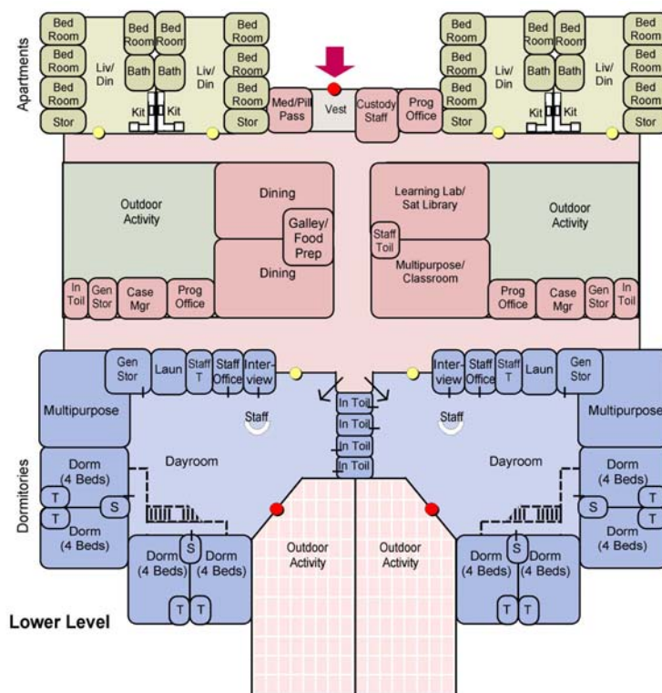
CDCR Reentry Facility Dormitory & Apartment Housing Diagram - Option 3 96 Capacity (2 Dorm Housing Units @ 32 Beds, 8 Apartments @ 4 Beds) ● secure access control ● secondary access control
